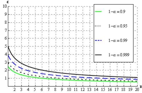
Fig. 10: Accuracy versus amount of sampling (i.e. n number of reviewers) for the most common values for the confidence probability. i.e. (1 - \alpha) = 0.9, 0.95, 0.99, 0.999 and using the computed approximation for the population standard deviation s_n = 1.51 in C1
