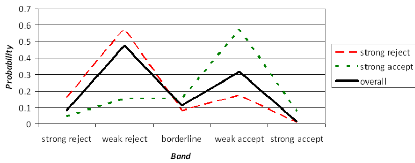
Fig. 6: Band Agreement for C2 (“fair” ICC agreement)
