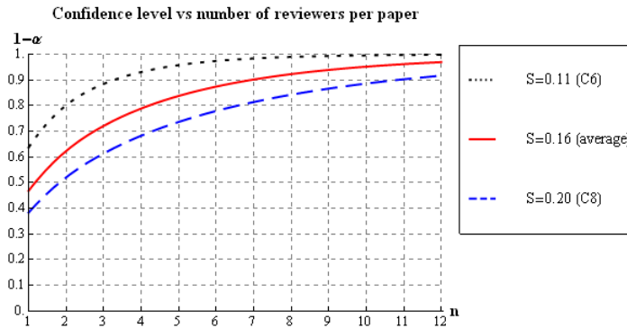
Fig. 13: Confidence level vs number of reviews per paper with error of the mark \varepsilon = 0.1
