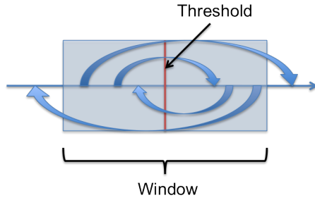
Fig. 3: Schema for the robustness analysis for a fixed window of papers and corresponding threshold. The rounded arrows indicate the types of relevant cases for a paper within the window to change its fate due to a perturbation on its marks.
