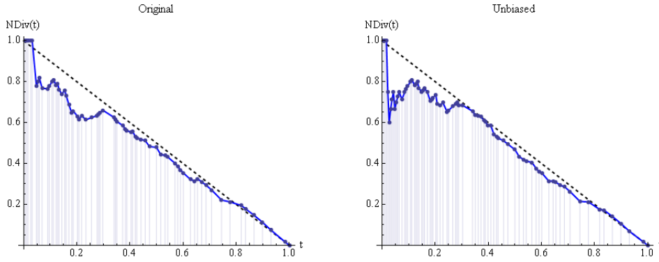
Fig. 8: Normalized divergence between original and citations-based rankings for conference C1 for all accepted papers: (a) on the left, peer-review ranking vs. citation-based ranking on the left; (b) on the right, peer-review-unbiased ranking vs. citation-based ranking.
