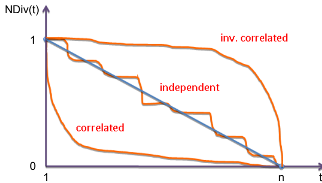
Fig. 1: Examples of different divergence curves. The index t in the X axis represents the top t contributions that are considered by the divergence. The Y axis shows how many items among the top t in the first ranking are also among the top t in the second ranking. The Divergence values (Y axis) are normalized by t .
