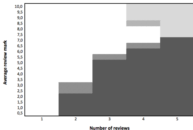
Fig. 14: Deterministic and statistical acceptance and rejection analysis for a contribution. Dark areas at the bottom: 100% rejected. Shaded areas at the top: 100% accepted. Dashed areas top/bottom: 95% probability accepted/rejected
