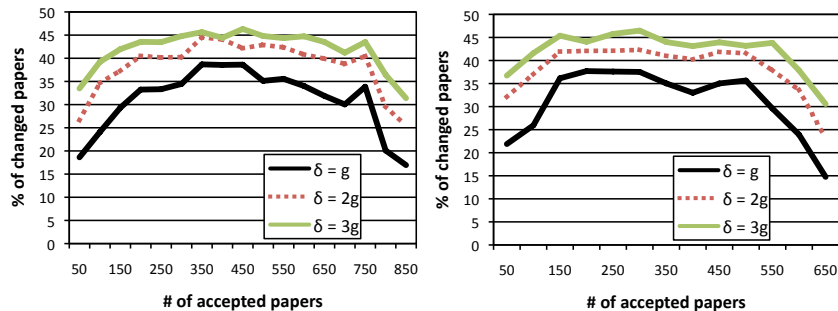
Fig. 4: Robustness curves for conferences C1 (left) and C3 (right) with fixed sliding window = 100 observations. Granularity is g = 1 for C1 and g = 0.5 for C3. The x-axis shows the (variable) number of accepted paper used in the computation
