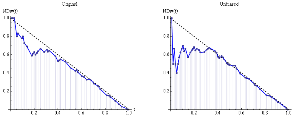
Fig. 9: Normalized divergence between original and citations based rankings for conference C1 for the top 50% accepted papers : (a) on the left, peer-review ranking vs. citation-based ranking on the left; (b) on the right, peer-review-unbiased ranking vs. citation-based ranking.
