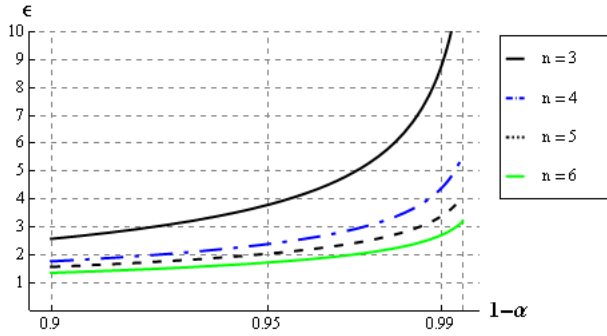
Fig. 11: Accuracy of estimation versus confidence probability depending on the considered number of marks n .
