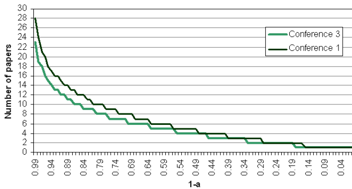
Fig. 16: Number of papers per reviewer for different values of 1-\alpha ( 0.99 \leq 1-\alpha \leq 0.01 )
