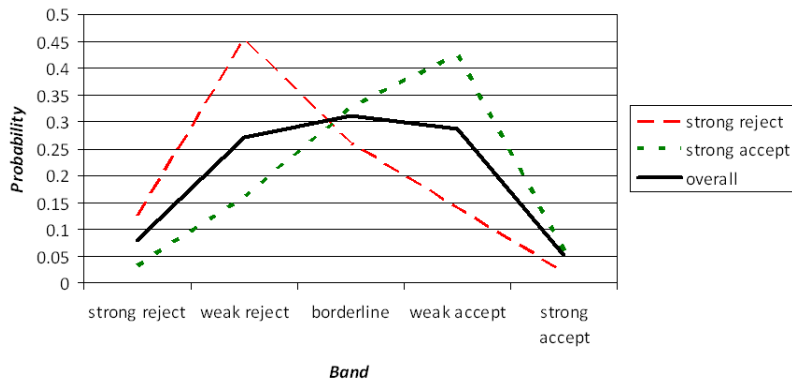
Fig. 5: Band Agreement for C1 (“high” ICC agreement)
