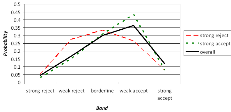
Fig. 7: Band Agreement for C3 (“low” ICC agreement)
